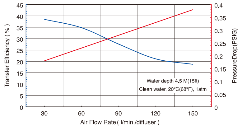
BHB-MD225 Fine Bubble Membrane Diffuser Performance Curve
